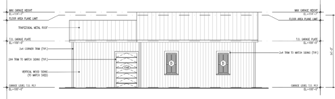
04 NORTH ELEVATION - GARAGE
