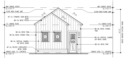
02 NORTH ELEVATION - GARAGE
