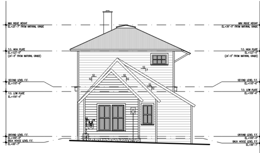
02 SOUTH ELEVATION - EXISTING SCALE: 1/8"=1'-0"
