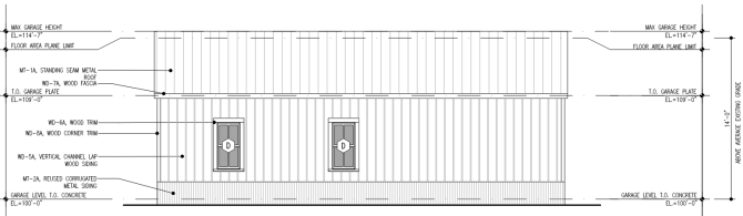
03 EAST ELEVATION - GARAGE
