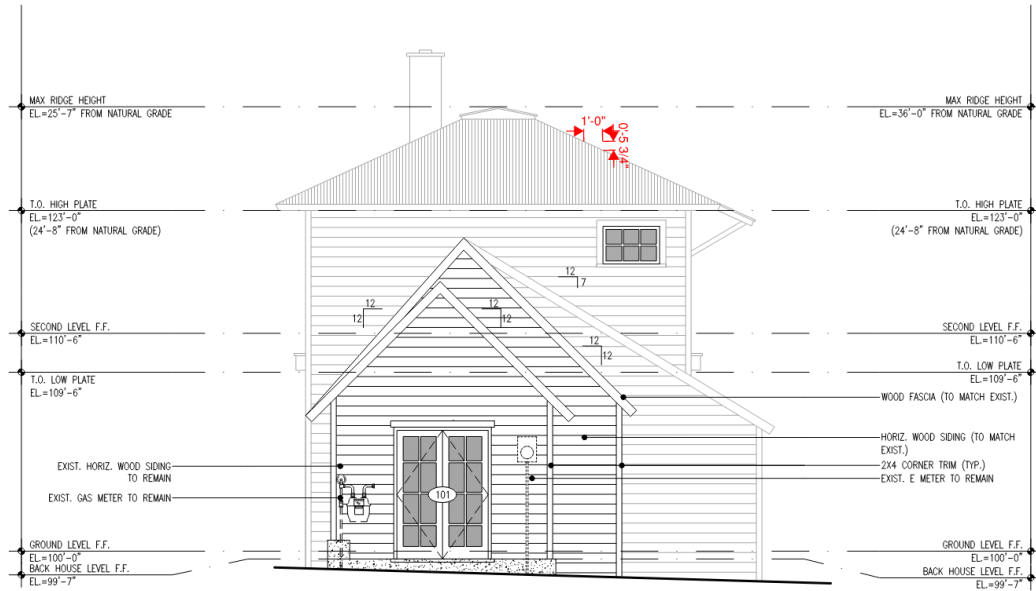
02 SOUTH ELEVATION - PROPOSED SCALE: 1/4"=1'-0"
