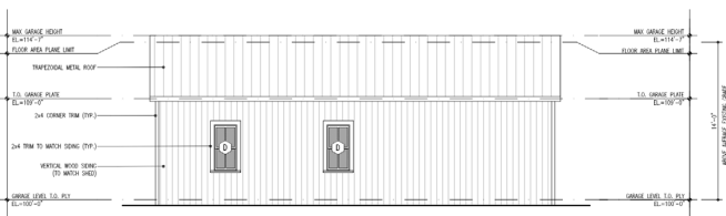
03 SOUTH ELEVATION - GARAGE
