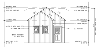
02 EAST ELEVATION - GARAGE
