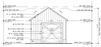
01 SOUTH ELEVATION - GARAGE
