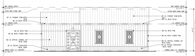
04 WEST ELEVATION - GARAGE
