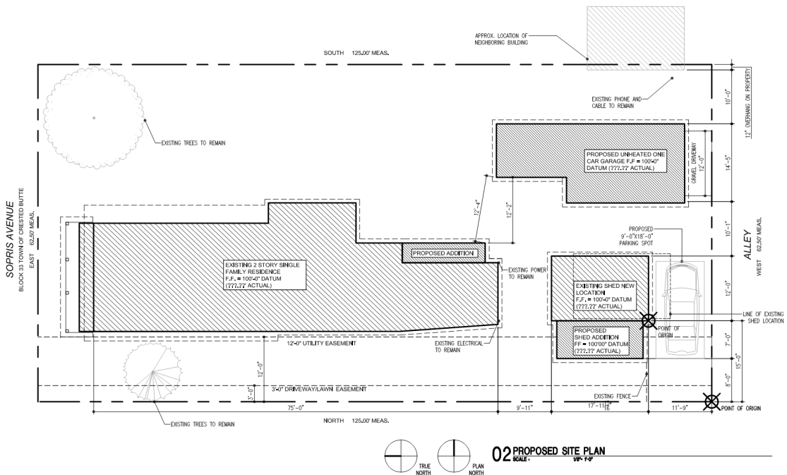
1/21 DRC: Proposed Site Plan
